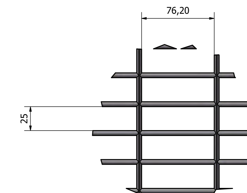
MESH SIZE
