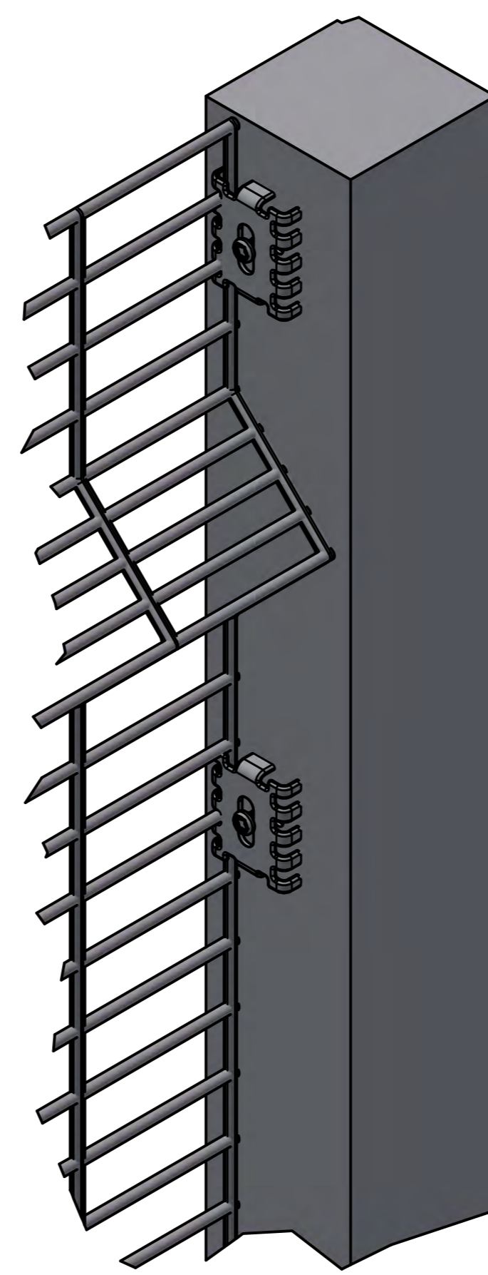
CLAMP DETAIL
